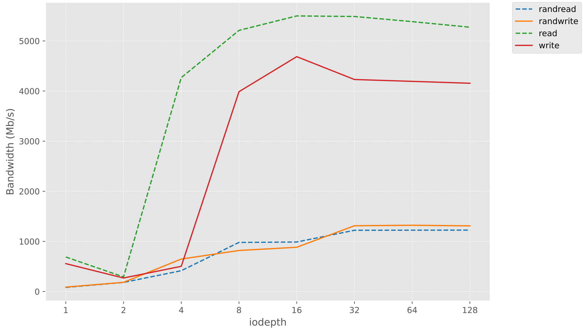
Bandwidth vs iodepth
